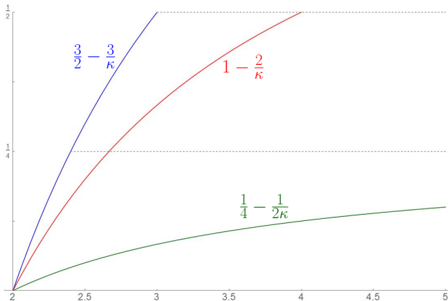
FIGURE 1. A comparison of the different polynomial exponents that appear in Theorems 1.3–1.5. The dotted lines are at height 1/4 and 1/2.
