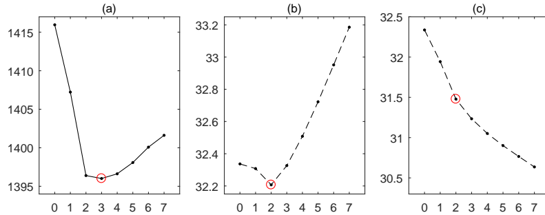
FIG 6. (a)–(b): Plots of the penalized objective function based on segmentation, corresponding to equations (8)–(9), versus the number of change-points L , respectively. (c): Plot of \mathcal{S}_{\hat{\mathcal{B}}}(\hat{\tau}_{L,1}^{(2)}, \dots, \hat{\tau}_{L,L}^{(2)}) + L\hat{Q}_{\hat{\mathcal{B}}}(55, 90) versus the number of change-points L .
