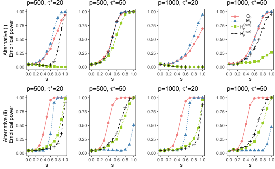
FIG 3. Comparison of size-corrected empirical power under the alternative hypotheses (i) and (ii).
