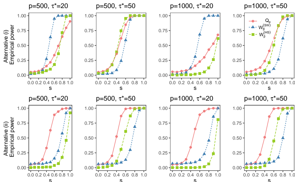
FIG 2. Comparison of empirical power for the proposed Q_{p,\hat{s}} test, W_{\hat{p}}^{(SW)} by Srivastava and Worsley (1986) and W_{\hat{p}}^{(HS)} by Horváth and Serbinowska (1995) under the alternative hypothesis (i) with \omega = 0.3 , and the alternative hypothesis (ii) with \omega = 0.7 , where d = 6 .
