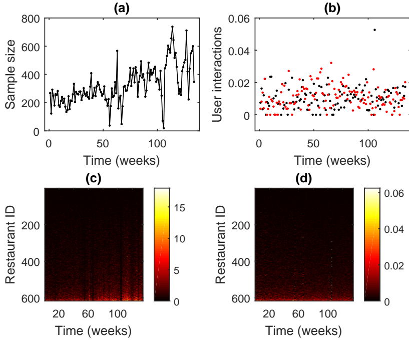
FIG 4. Description of the raw data over time. (a): Sample size over time; (b): Scatter plot of the proportions of two randomly chosen restaurants over 134 weeks; (c): Heatmap of user interactions of 617 restaurants with brightness representing the frequency of users' final choices; (d): Heatmap of the proportions allotted in all the restaurants with time.
