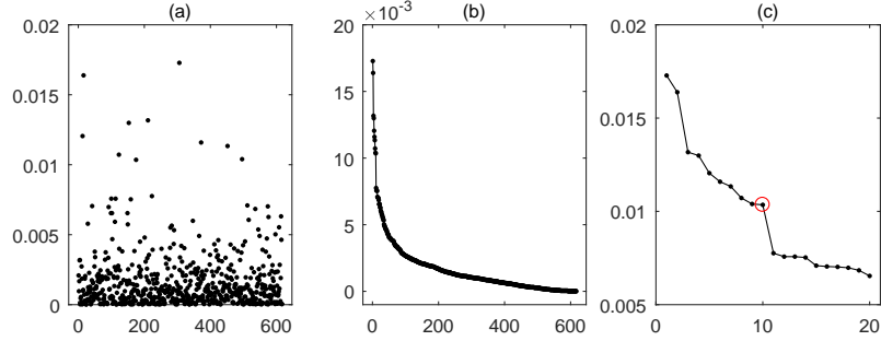
FIG 5. Estimation of the sparsity pattern. (a): Scatter plot of the estimated proportions \hat{q}_j 's for j = 1, \dots, p ; (b)–(c): Plots of the estimated proportions in a decreasing order, i.e., \hat{q}_{(j)} 's, for j = 1, \dots, p and j = 1, \dots, 20 , respectively.
