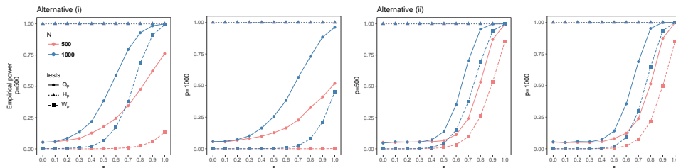
FIG 1. Comparison of empirical power at a 5% significance level for the two-sample homogeneity test under different (p, N) -settings and the alternative hypothesis (i) with \omega = 0.3 and the alternative hypothesis (ii) with \omega = 0.7 , where d = 6 . Here Q_p is short for Q_{p, \hat{\omega}} .
