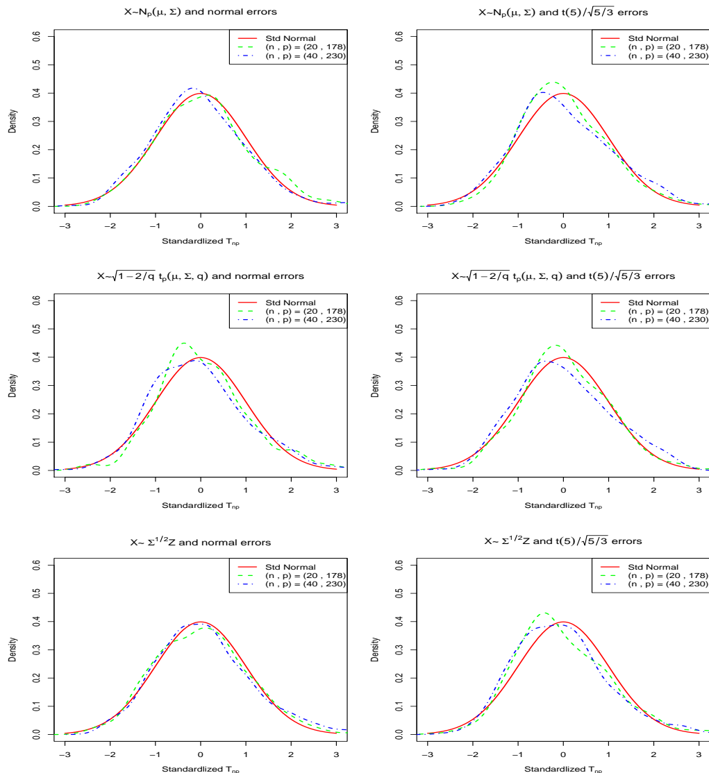
FIG 1. The asymptotic null distributions of the standardized UT test statistic T_{n,p} .
