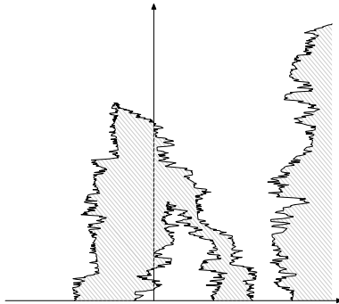
FIG 1. An illustration of the standard coloring \hat{m} of [0, \infty) \times \mathbb{R} induced by an initial configuration \mathbf{u}_0 with five interfaces and a regular annihilating system starting from \mathcal{I}(\mathbf{u}_0) . Type 1 is drawn in white and type 2 is shaded grey. The corresponding standard element (\hat{\mathbf{u}}_t)_{t \geq 0} \in \mathcal{C}_{[0, \infty)}(\mathcal{U}) is such that \hat{\mathbf{u}}_t^{(1)}(x) (resp. \hat{\mathbf{u}}_t^{(2)}(x) ) agrees with w_t(x) for all (t, x) in the white (resp. shaded) area and is zero otherwise.
