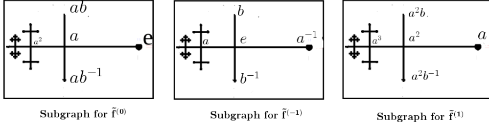
Figure 2. The \ell -subgraphs corresponding to \tilde{f}^{(\ell)} for \ell = 0, -1, 1
