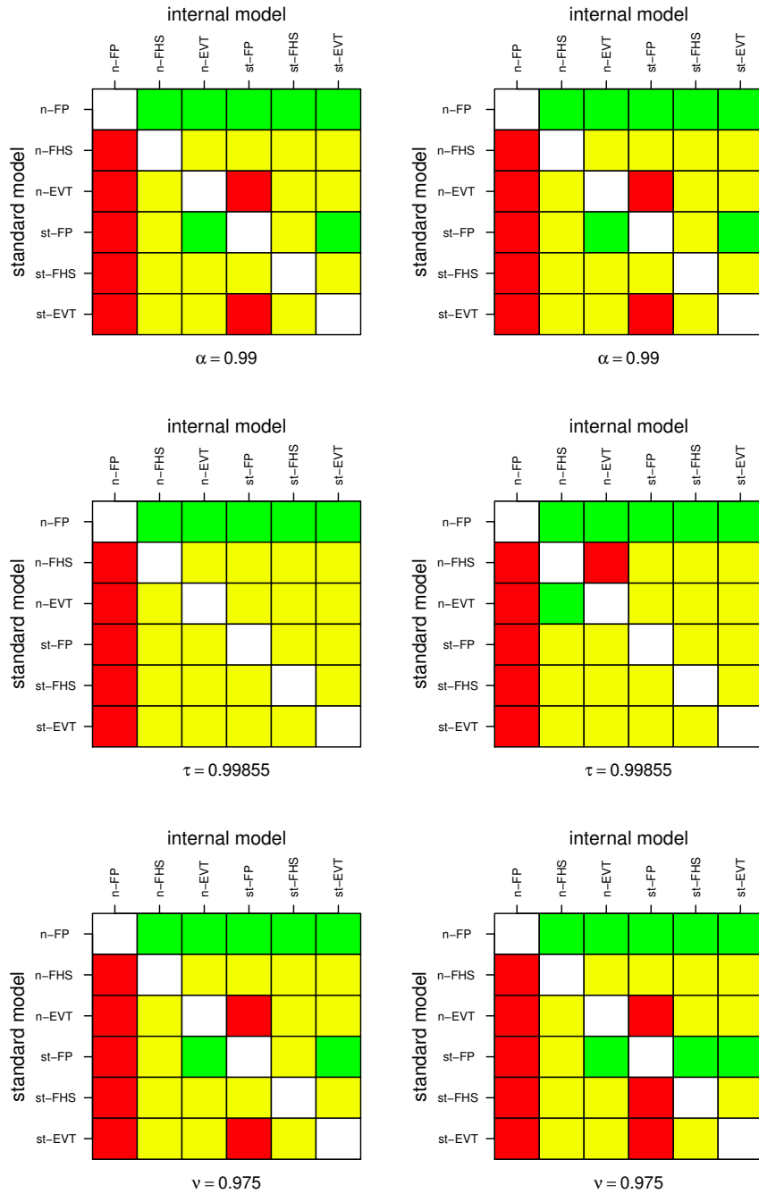
Figure 4: Traffic light matrices for \text{VaR}_{\alpha} (top row) based on scoring functions in (2.19) (left) and (2.20) (right), for \tau -expectile (middle row) based on scoring functions in (2.21) (left) and (2.22) (right), and for (\text{VaR}_{\nu}, \text{ES}_{\nu}) (bottom row) based on scoring functions in (2.23) (left) and (2.24) (right) at the test confidence level \eta = 0.05 , for the data analysis in Section 3.3.
