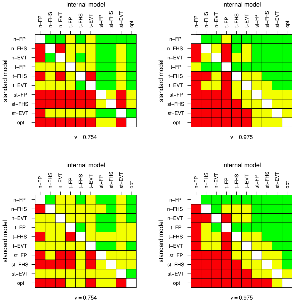
Figure 3: Traffic light matrices for (\text{VaR}_v, \text{ES}_v) forecasts at the test confidence level \eta = 0.05 . The top and bottom rows are based on the scoring functions in (2.23) and (2.24), respectively.
