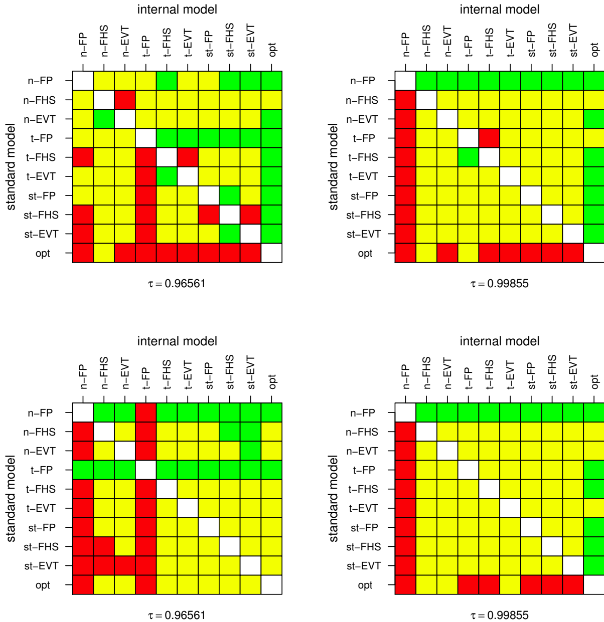
Figure 2: Traffic light matrices for \tau -expectile forecasts at the test confidence level \eta = 0.05 . The top and bottom rows are based on the scoring functions in (2.21) and (2.22), respectively.
