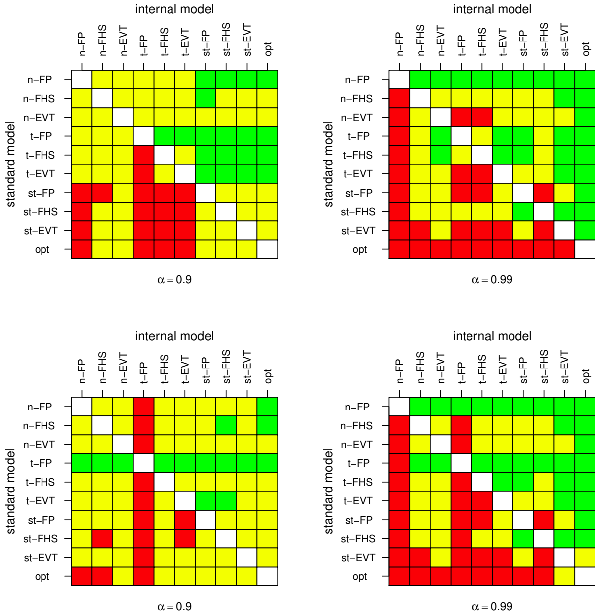
Figure 1: Traffic light matrices for VaR α forecasts at the test confidence level η = 0.05. The top and bottom rows are based on the scoring functions in (2.19) and (2.20), respectively.
