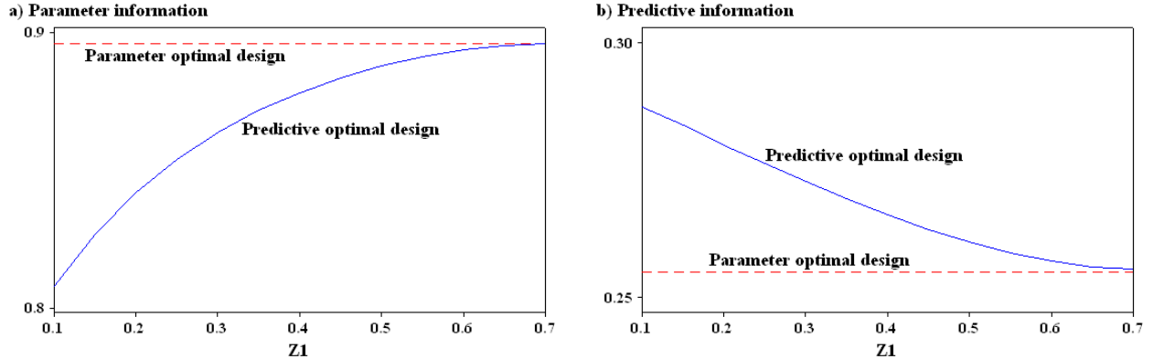
FIGURE 2: Parameter information per dimension M(\mathbf{Y}; \Theta | Z, \eta)/p and predictive information M(\mathbf{Y}; Y_\nu | Z, \mathbf{z}, \eta) under the predictive and parameter optimal designs against z_{\nu 1} , \mathbf{z}'_\nu \mathbf{z}_\nu = 1 for p = 2, n = 10, \eta = 1, v_{01} = v_{02} = 1 .
