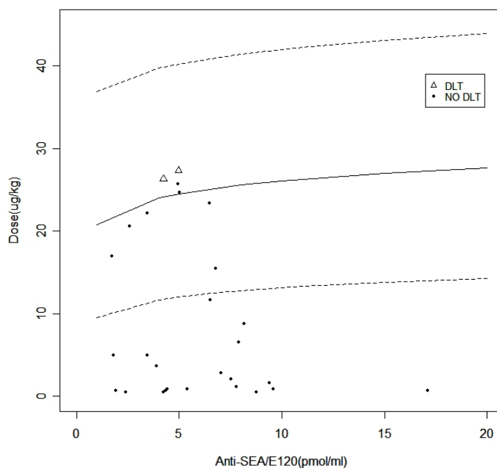
FIG 4. Dose allocation as a function of baseline Anti SEA/E120 during the trial for all 28 NSCLC & PC patients. The solid line is the MTD conditional on the covariate Anti SEA/E120 which corresponds to the posterior median of the conditional posterior distribution of the MTD and the dashed lines delimit the 95% Bayesian credible region.
