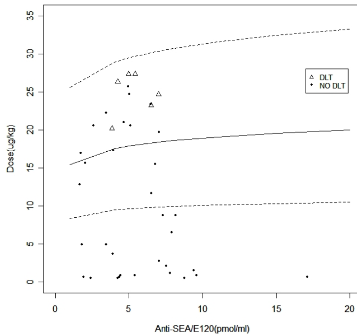
FIG 3. Dose allocation as a function of baseline Anti SEA/E120 during the trial for all 39 patients. The solid line is the MTD conditional on the covariate Anti SEA/E120 which corresponds to the posterior median of the conditional posterior distribution of the MTD and the dashed lines delimit the 95% Bayesian credible region.
