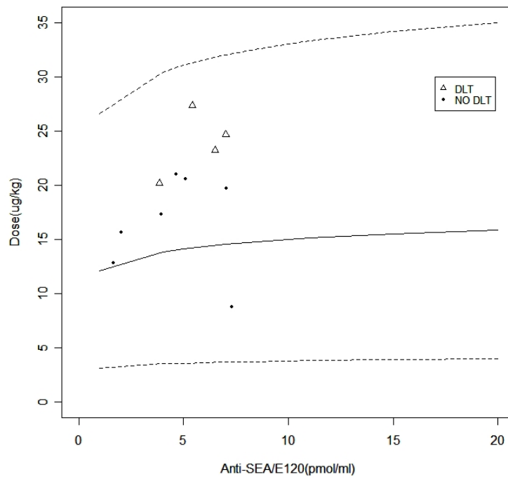
FIG 5. Dose allocation as a function of baseline Anti SEA/E120 during the trial for all 11 RCC patients. The solid line is the MTD conditional on the covariate Anti SEA/E120 which corresponds to the posterior median of the conditional posterior distribution of the MTD and the dashed lines delimit the 95% Bayesian credible region.
