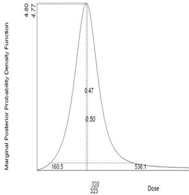
FIG 2. Posterior density of the MTD after 33 patients have been treated. The posterior mode is 323 (47th percentile) and the median and dose to be given to the 34th patient is 328. The 95% highest posterior density interval is [160.5, 536.1].
