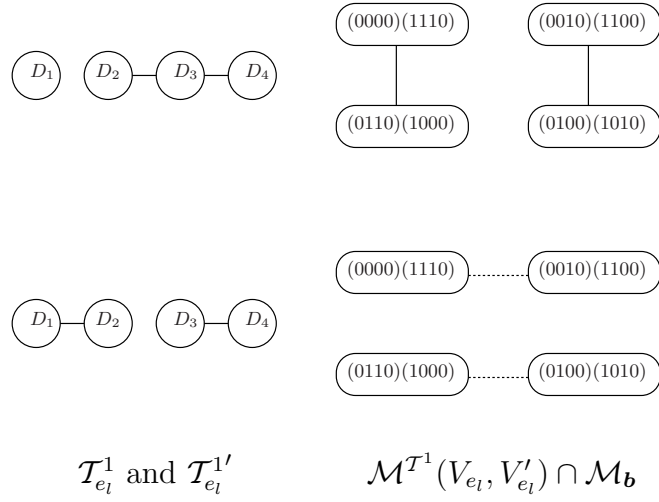
Figure 8: The structure of \mathcal{M}_b^{T^1}
