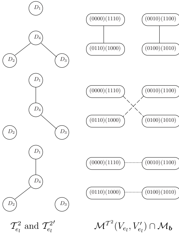
Figure 9: The structure of \mathcal{M}_b^{T^2}
