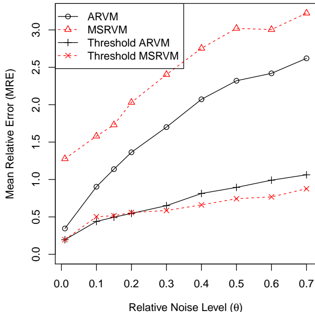
Figure 1: The MRE plots of the four estimators for n = 200 and p = 100 .
