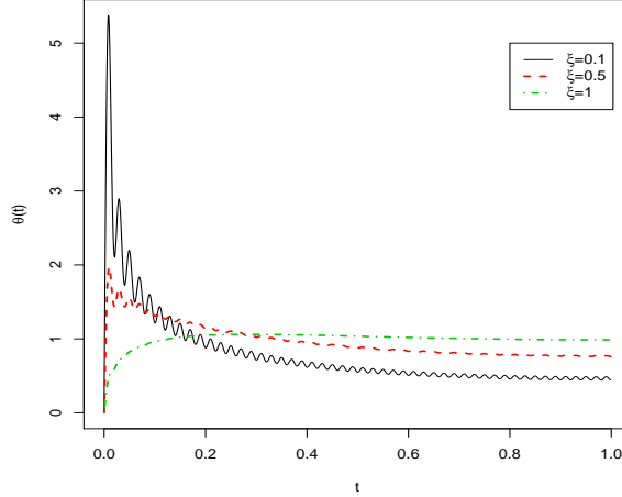
FIGURE 1. Three functions \theta in \Theta_{KL} when B = 1 .
