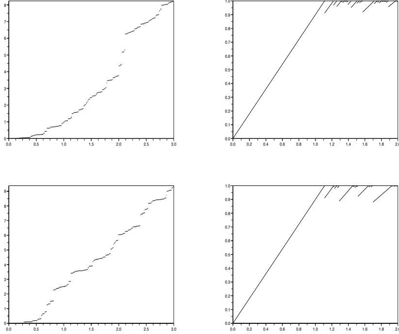
FIG 1. Two sample paths of the stochastic process M built using the function \gamma(y) := \min(1/2 + y/4, 0.9) . On the right hand-side are plotted the theoretical spectra D_M([0, 3], \cdot) .
