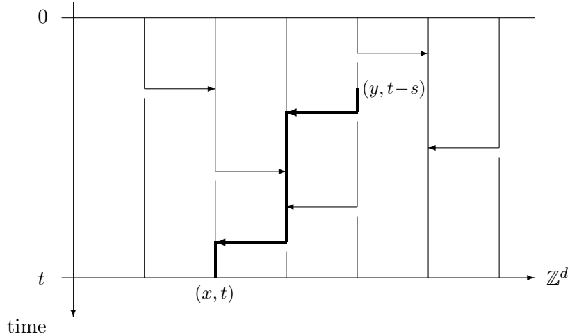
Fig. 2: Dual graphical representation \mathcal{G}_t^* . Opinions propagate along time-reversed coalescing paths.
