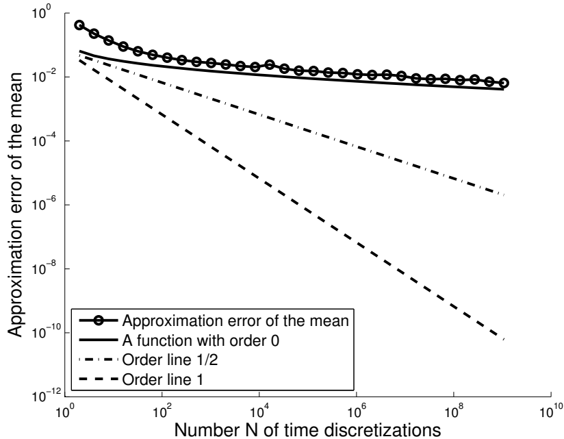
Figure 1: The norm \|\mathbb{E}[X(T)] - \mathbb{E}[Y^{\frac{T}{N}}(T)]\| of the difference between the mean of the solution of the SDE (107) and the mean of the Euler-Maruyama approximations (109) for T = 2 and N \in \{2^1, 2^2, \dots, 2^{29}, 2^{30}\} . The function with convergence order 0 is given by (121).
