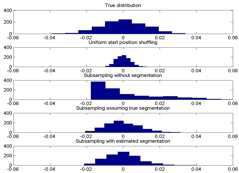
Fig 3. Comparison of different subsampling schemes
