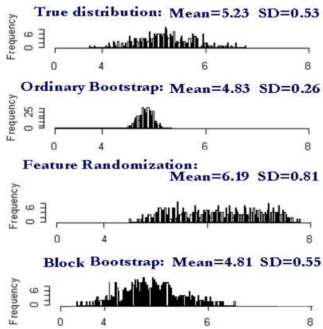
Fig 1. Comparison of different subsampling schemes
