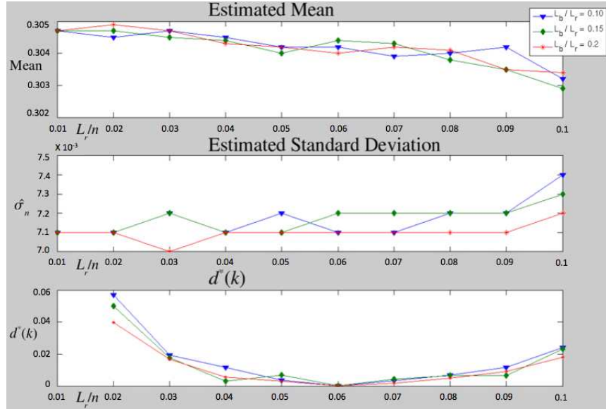
Fig 4. Comparison of block subsampling distributions
