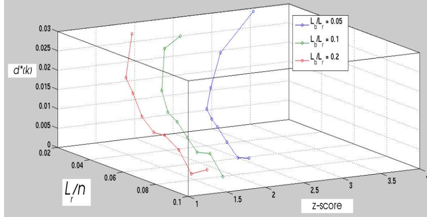
Fig 7. The relationship between the estimated z-score, d^*(k) , L_r and L_b . As L_r increases, our estimate of \hat{\sigma}_n (not shown) increases, which drives the estimated z-score down. As L_r becomes too small, we lose the stability of our estimates, and d^*(k) increases. For the smallest value of L_r shown here, the estimated z-score increases sharply, but the corresponding value of d^*(k) indicates that this parameterization is unreliable. The ideal parameterization under d^*(k) is given by L_r/n = 0.09 and L_b/L_r = 0.20 .
