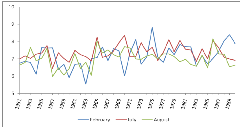
FIG. 2. Time series plot of log transformed data on mean monthly water discharges of the Nacetinsky creek for the months of February, July, and August for the years 1951-1990.
