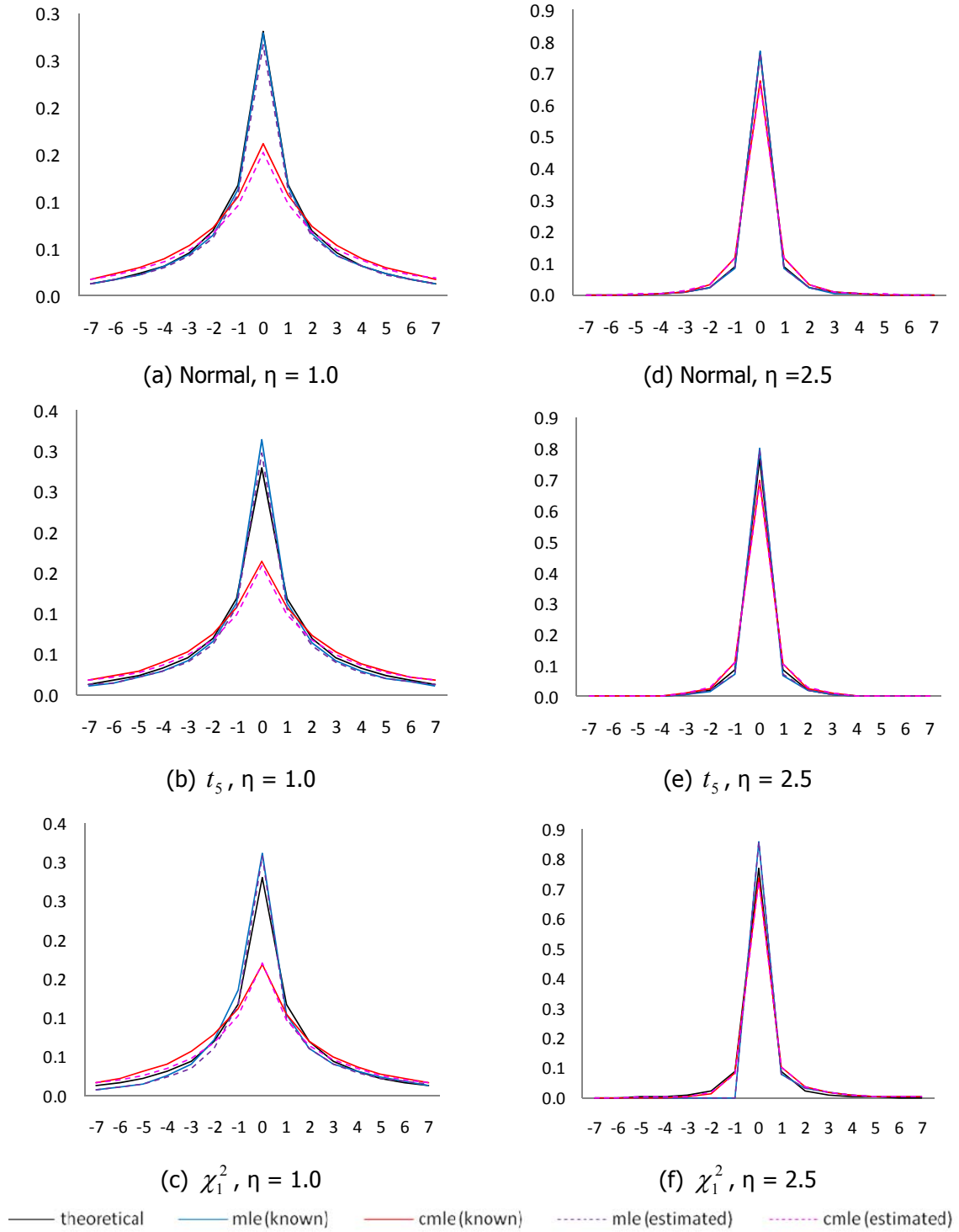
FIG. 1. Plots of theoretical mle, empirical mle (known), empirical mle (estimated), empirical cmlc (known), empirical cmlc (estimated) distributions of the centered change-point when n = 100, \tau = 50 under normal (a); t_5 (b) and \chi_1^2 (c) when \eta = 1.0 ; and normal (d); t_5 (e) and \chi_1^2 (f) when \eta = 2.5 .
