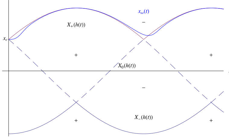
Figure 3: The function x_\omega(t) (blue line) for small values of \omega tracks the positive branch X_+(h(t)) (black line).
