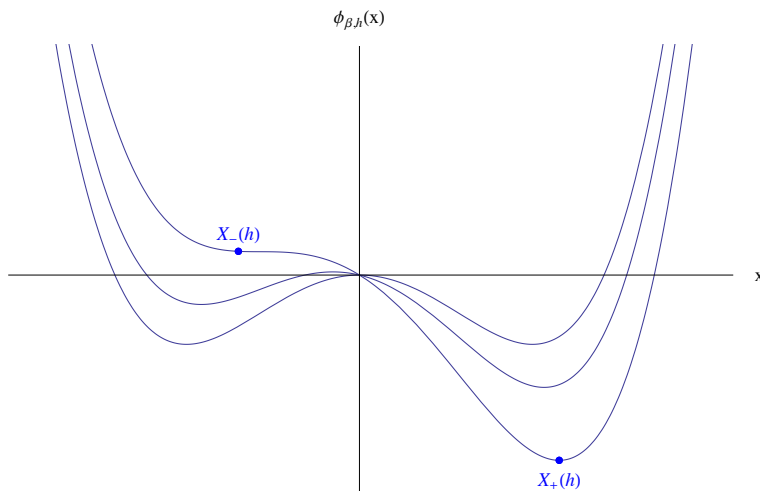
Figure 2: The picture shows some profiles of \phi_{\beta,h}(x) according to different values of h , for \beta > 1 .
