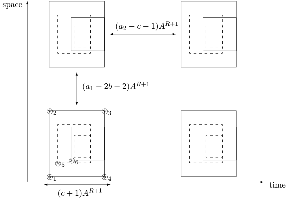
Figure 2: The dashed blocks are R -blocks, i.e., B_R^A(x, k) (inner) and \tilde{B}_R^A(x, k; b, c) (outer) for some choice of A, x, k, b, c . The solid blocks are (R + 1) -blocks, i.e., B_{R+1}^A(y, l) (inner) and \tilde{B}_{R+1}^A(y, l; b, c) (outer) for a choice of A, y, l, b, c such that they contain the corresponding R -blocks. Furthermore, \{\otimes_i\}_{i=1,2,3,4,5,6} represents the space-time coordinates \otimes_1 = ((y - 1 - b)A^{R+1}, (l - c)A^{R+1}) , \otimes_2 = ((y + 1 + b)A^{R+1}, (l - c)A^{R+1}) , \otimes_3 = ((y + 1 + b)A^{R+1}, (l + 1)A^{R+1}) , \otimes_4 = ((y - 1 - b)A^{R+1}, (l + 1)A^{R+1}) , \otimes_5 = ((x - 1 - b)A^R, (k - c)A^R) and \otimes_6 = ((y - 1)A^{R+1}, lA^{R+1}) .
