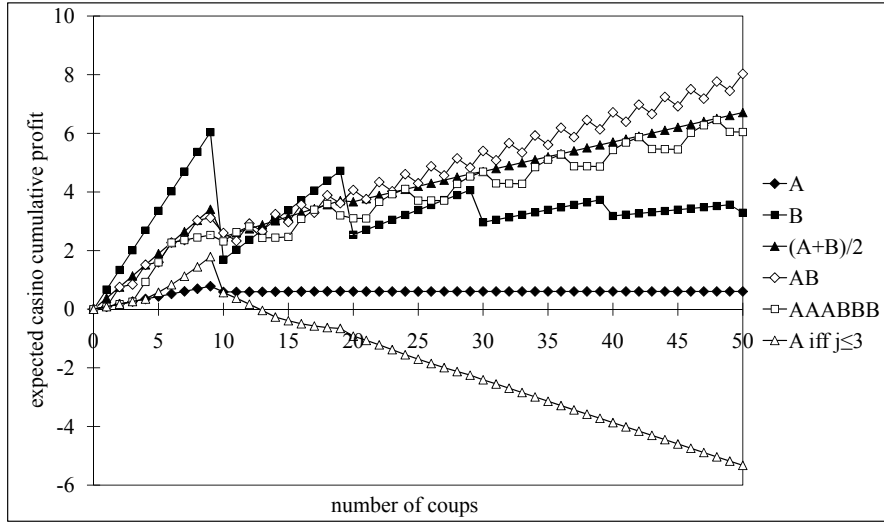
FIG 1. Expected casino cumulative profit for various player strategies. We assume a two-armed slot machine with hit frequencies p_A = 3/10 and p_B = 1/15 ; Futurity award paid after J = 10 consecutive losses, regardless of the order of play of the two arms; initial pointer position 0; and both arms fair when played exclusively ( \mu_A^* = \mu_B^* = 1 ). j is the Futurity pointer position. Results are by direct calculation (not simulation).
