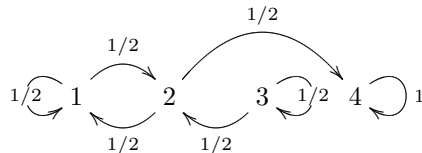
Figure 2: Graph structure for \tilde{K} .
