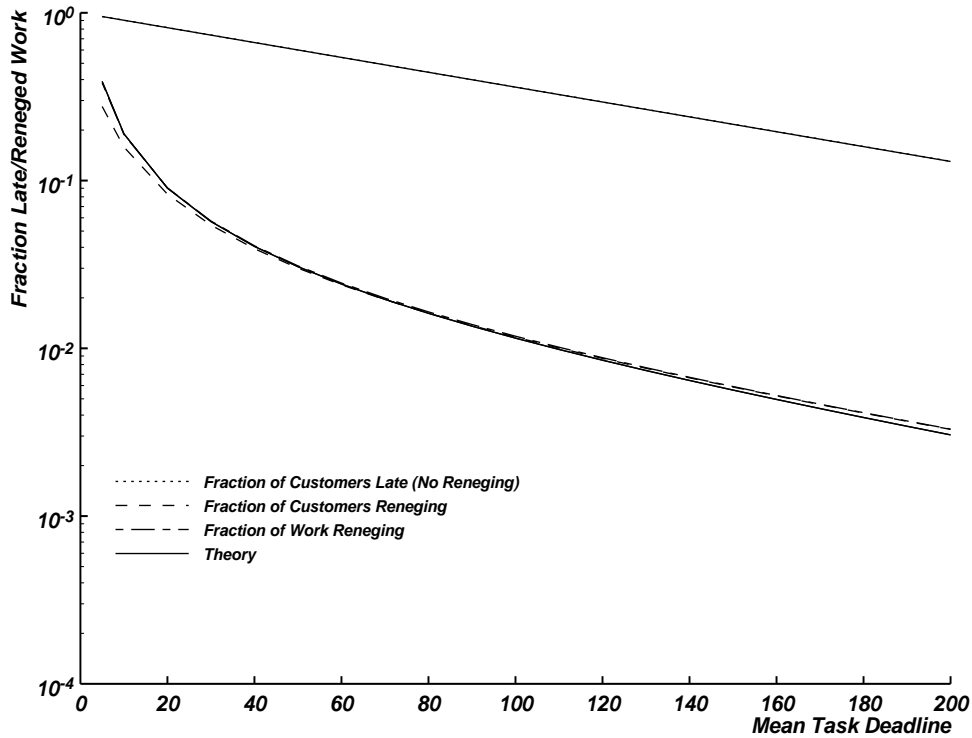
Figure 1: M/M/1 Queue
