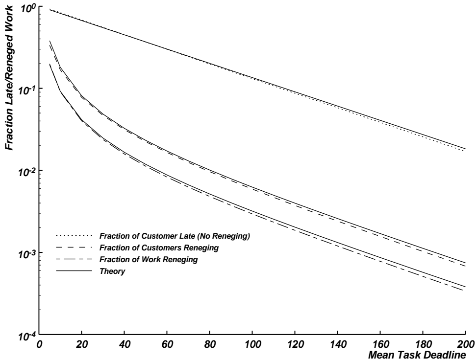
Figure 2: M/D/1 Queue
