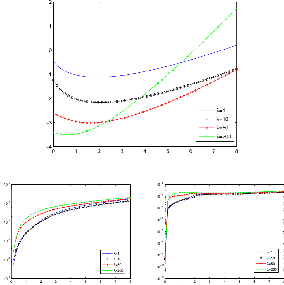
FIGURE 2. In this figure we fixed the standard deviation to \sigma = 0.25 and the rate parameter to \nu = 0.125 . The first row gives the barriers for the killing parameters \lambda = 1, 10, 50, 200 . The first and second panels in the second row give the relative errors for the survival function (resp. the hazard function).
