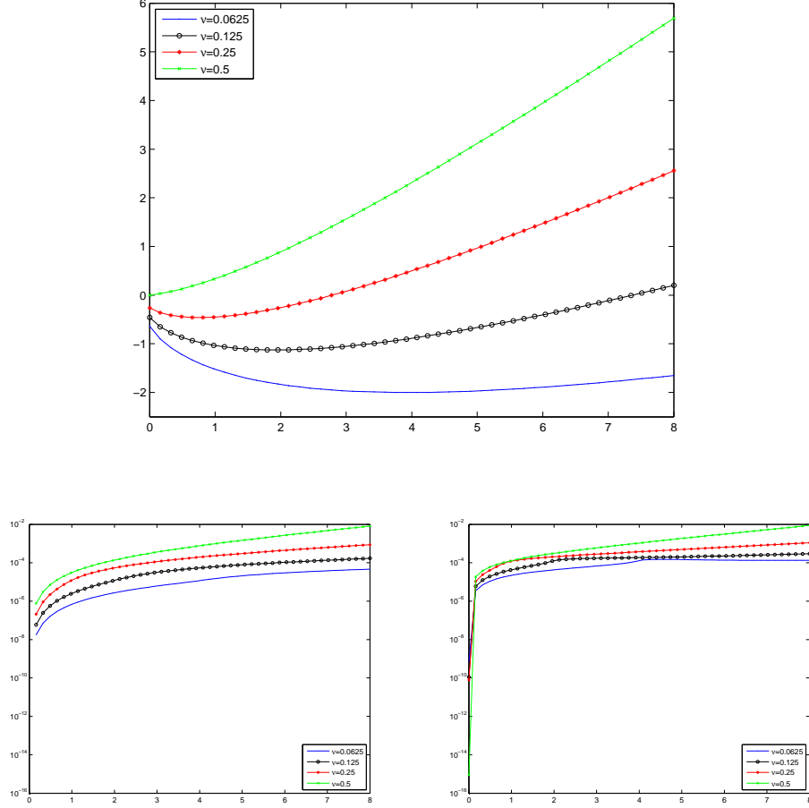
FIGURE 1. This figure displays the results of the numerical experiments described in Section 6. We fix the standard deviation for the initial distribution of the credit index process Y to be \sigma = 0.25 and the killing parameter to be \lambda = 1 . The first row gives the barriers for the rate parameters \nu = 0.0625, 0.125, 0.25, 0.5 of the exponential default time distribution. The first (resp. second) panels in the second row give the relative errors between the actual survival function values G(t) (resp. the actual hazard function values -g(t)/G(t) ) and the numerically computed ones – see the text for details.
