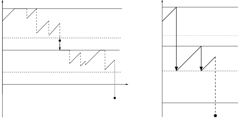
FIGURE 2. Illustrated in the figure on the left is a path of the risk process U^\pi in the absence of transaction cost ( K = 0 ) for a three-bands strategy with the lowest level b_1^+ equal to zero. The figure on the right pictures a path of the risk process U^\pi in the case K > 0 and \pi is a two-bands strategy with b_2^- = b_1^- . The vertical dashed stretches represent the claims, while lump sum dividend payments are indicated by arrows. At the moment \tau of ruin a penalty payment w(U_\tau) is required that is a function of the shortfall U_\tau
