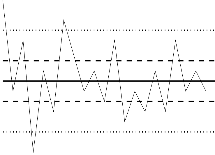
FIGURE 1. The martingale increments commence when X enters the inner band (dashed) and stop when X leaves the outer band (dotted).
